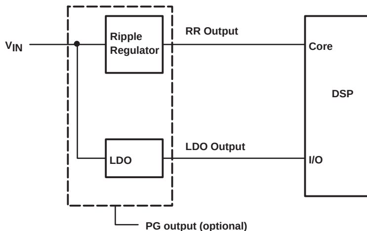
Figure 33. TPS56300 For On/Off Control DSP Application
